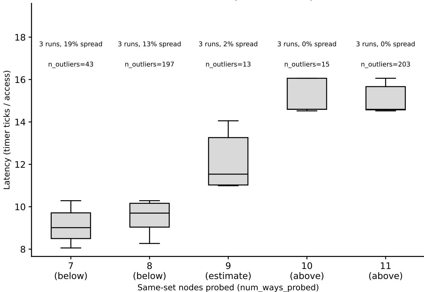
hazel_icelake_6326: associativity box plots, L1, random pattern (whiskers = p5/p95) (Phase I timing-only, auto pipeline) detected associativity estimate: 9-way
