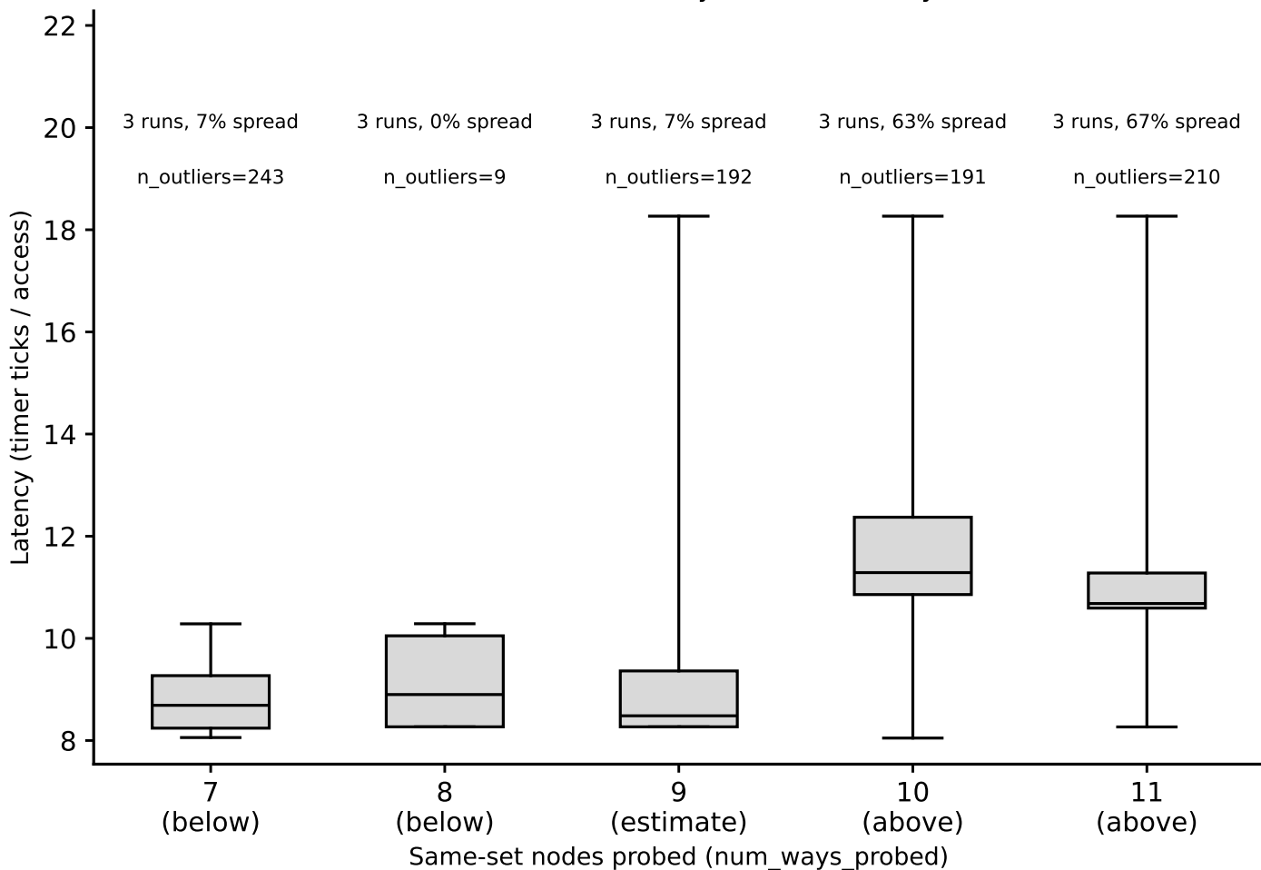
hazel_icelake_6326: associativity box plots, L3_LLC, random pattern (whiskers = p5/p95) (Phase I timing-only, auto pipeline) detected associativity estimate: 9-way
