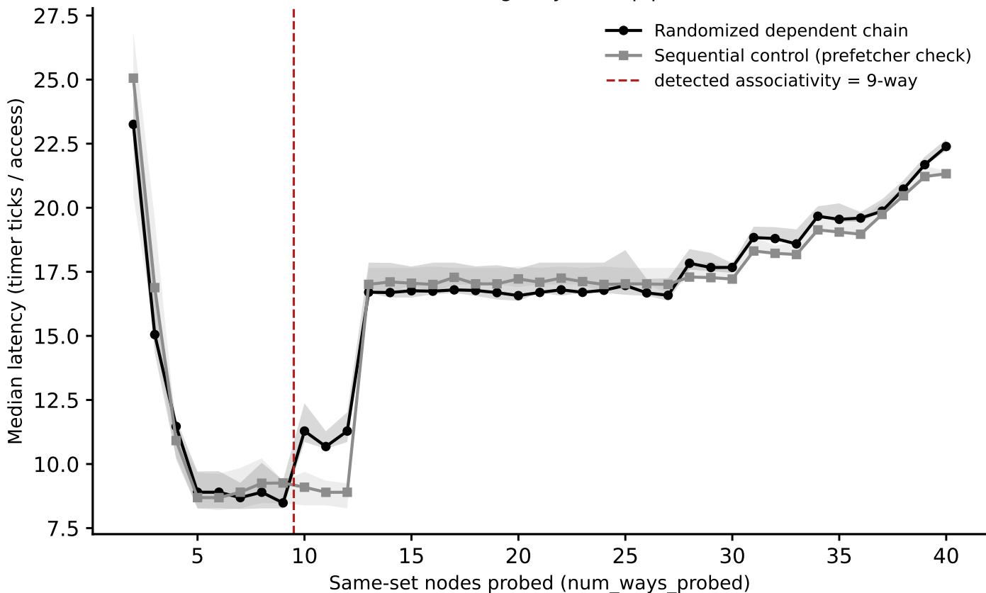
hazel_icelake_6326: associativity sweep, L3_LLC (stride=24.6758 MiB) (Phase I timing-only, auto pipeline)
