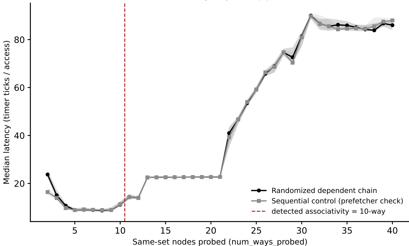
hazel_icelake_8358: associativity sweep, L3_LLC (stride=48 MiB) (Phase I timing-only, auto pipeline)
