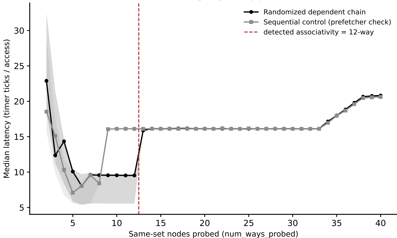
hazel_sapphirerapids: associativity sweep, L3_LLC (stride=38.0547 MiB) (Phase I timing-only, auto pipeline)
