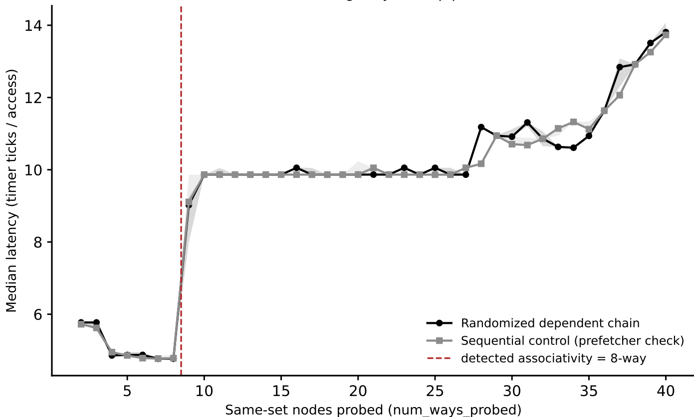
hazel_skylake: associativity sweep, L3_LLC (stride=22.6289 MiB) (Phase I timing-only, auto pipeline)
