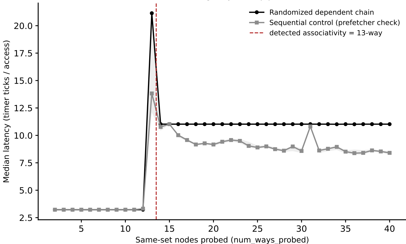
hazel_turin: associativity sweep, L2 (stride=1 MiB) (Phase I timing-only, auto pipeline)
