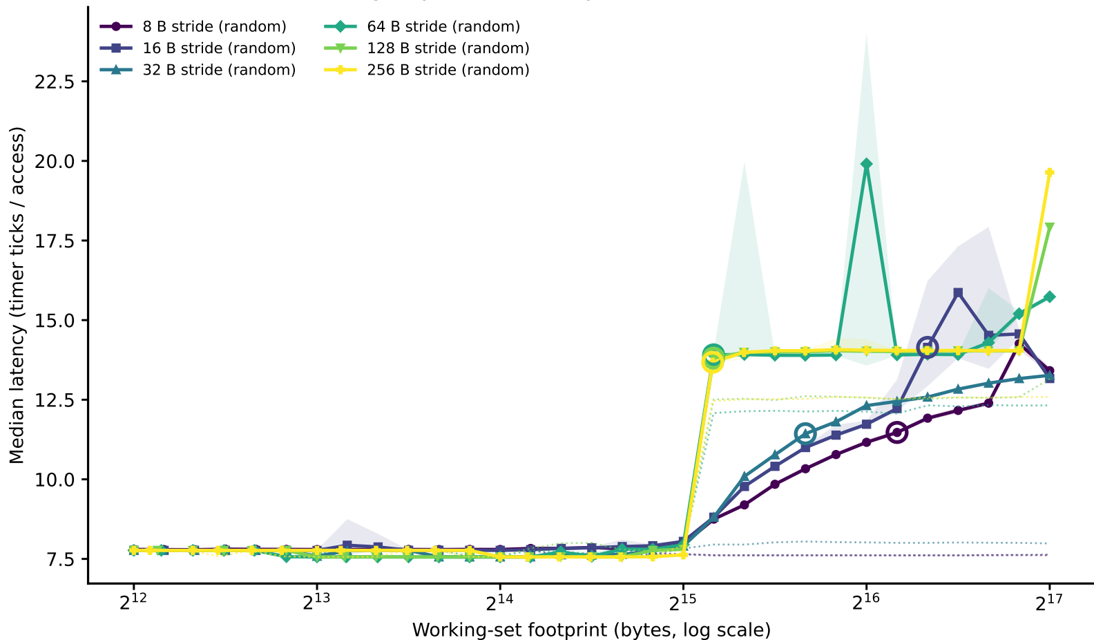
charnwood: line-size family of curves (dependent pointer chase) (Phase I timing-only, level boundary=32768B window=[4096,131072])
