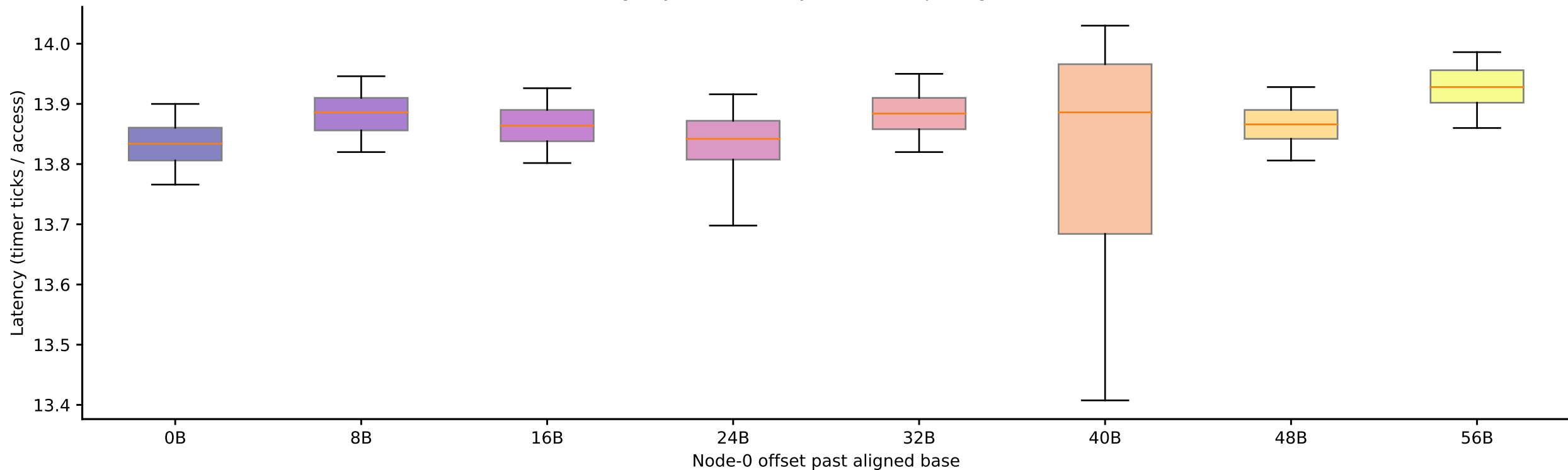
charnwood: candidate stride 64 B at footprint 35.875 KiB, by offset (Phase I timing-only, level boundary=32768B, step-4 alignment refinement)
