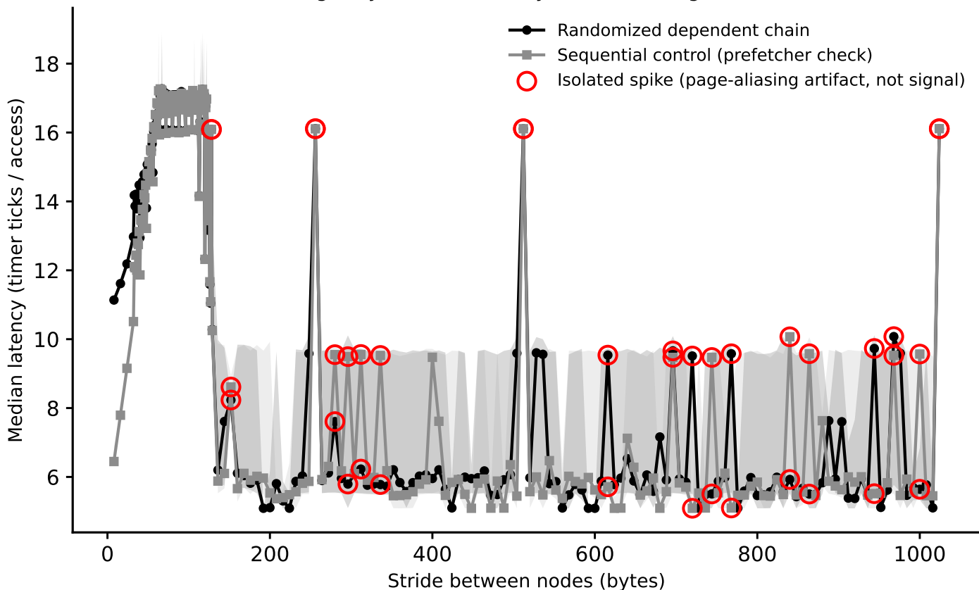
artemisia: line-size sweep (dependent pointer chase), footprint=96 KiB (Phase I timing-only, level boundary=49152B, single-curve method)
