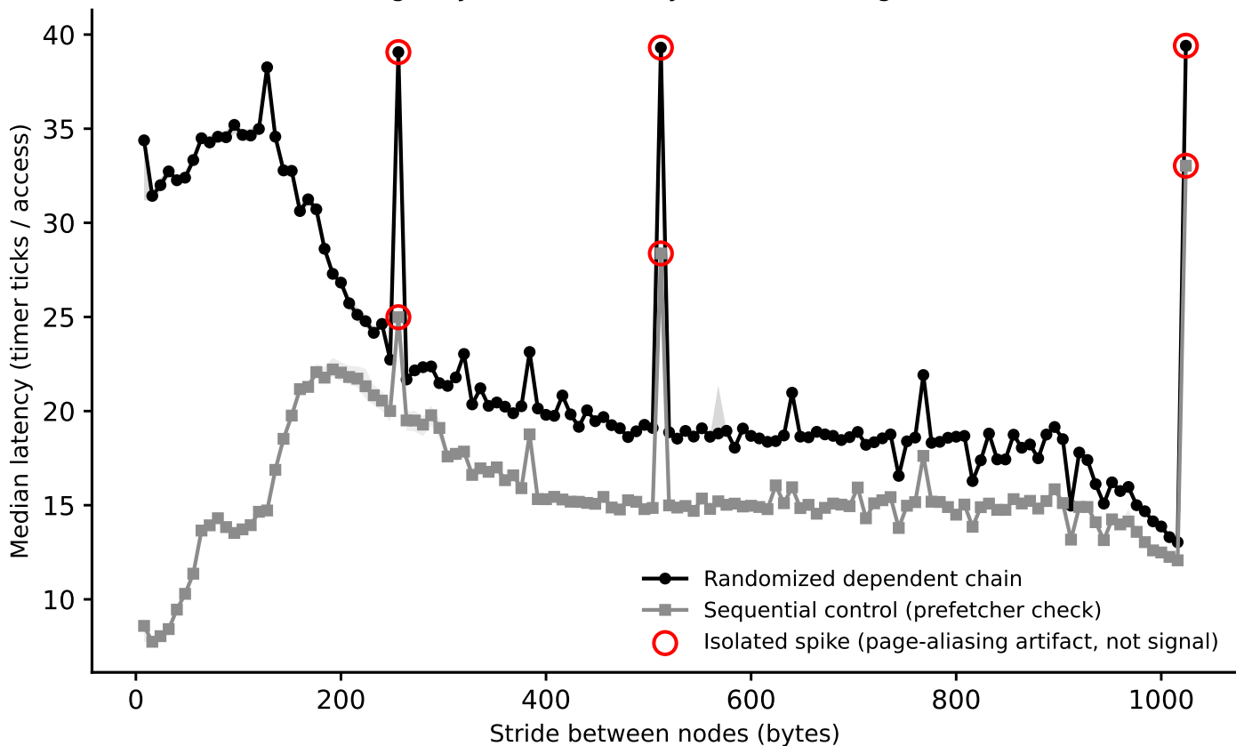
charnwood: line-size sweep (dependent pointer chase), footprint=512 KiB (Phase I timing-only, level boundary=262144B, single-curve method)
