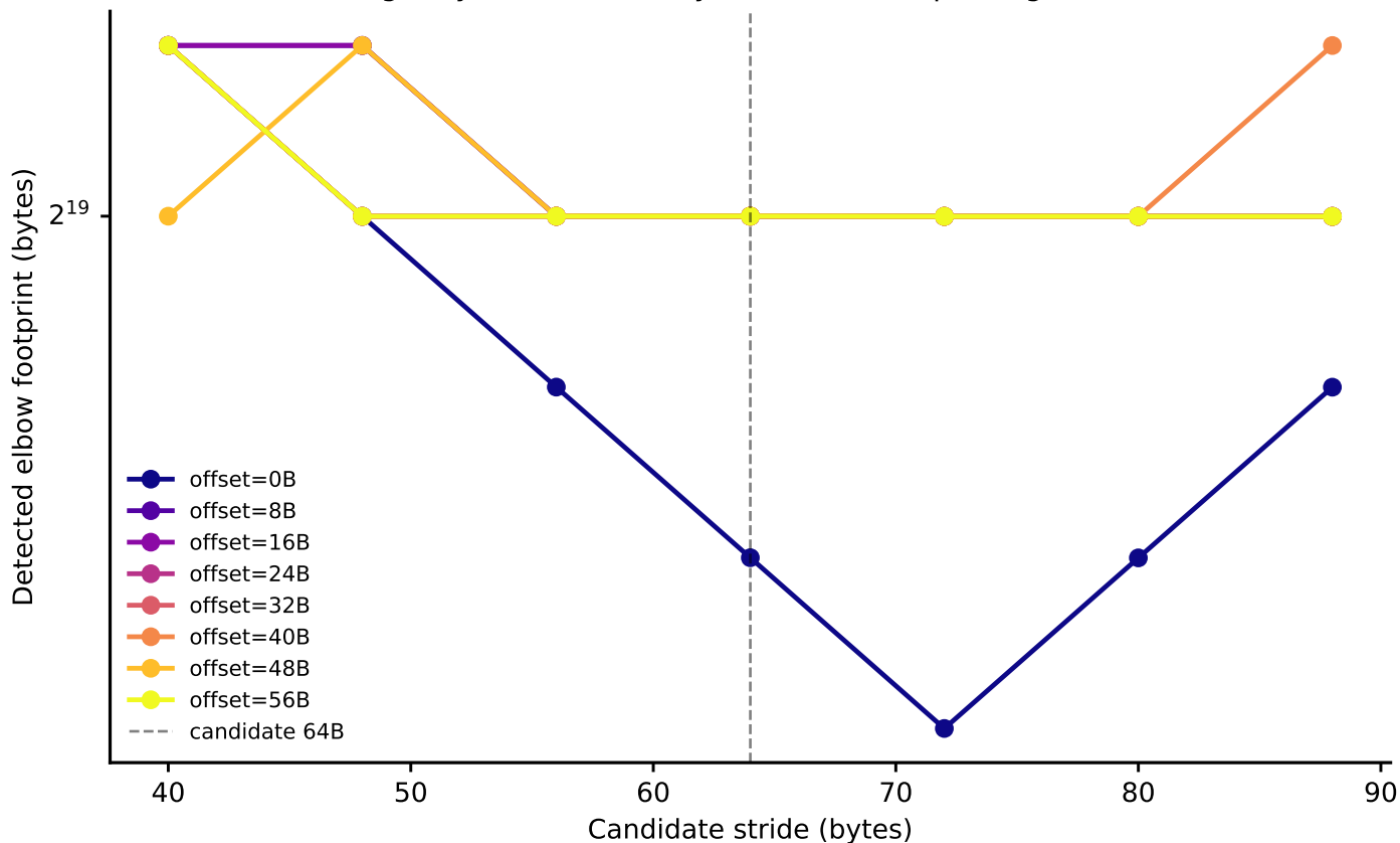
charnwood: line-size elbow vs. stride, by node-0 offset (Phase I timing-only, level boundary=262144B, step-4 alignment refinement)
