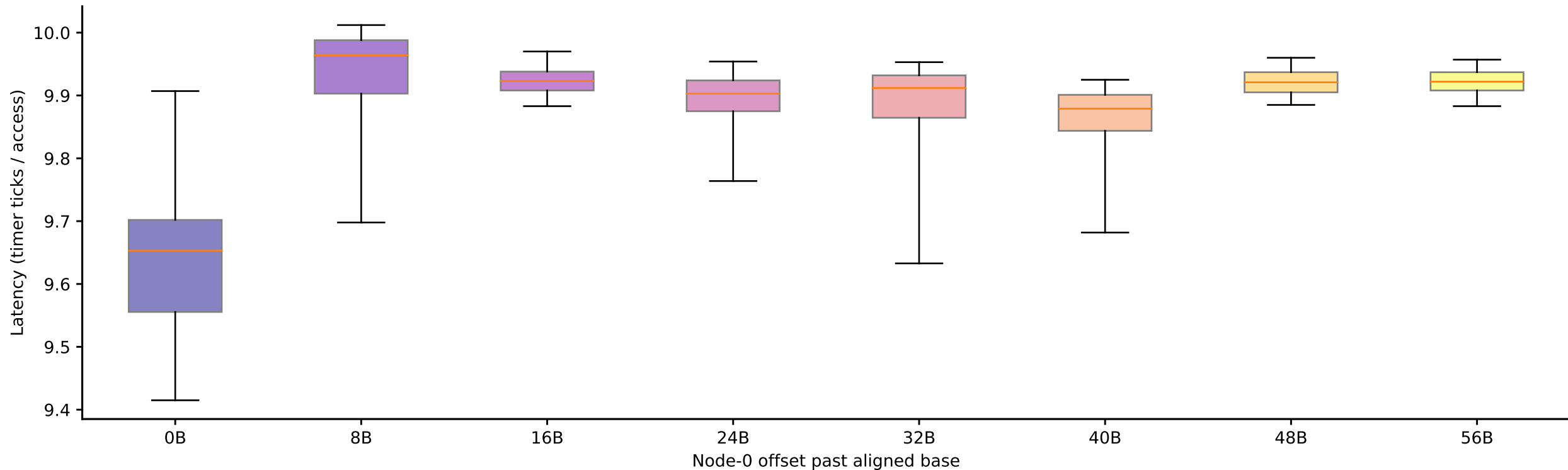
crux: candidate stride 64 B at footprint 35.875 KiB, by offset (Phase I timing-only, level boundary=32768B, step-4 alignment refinement)
