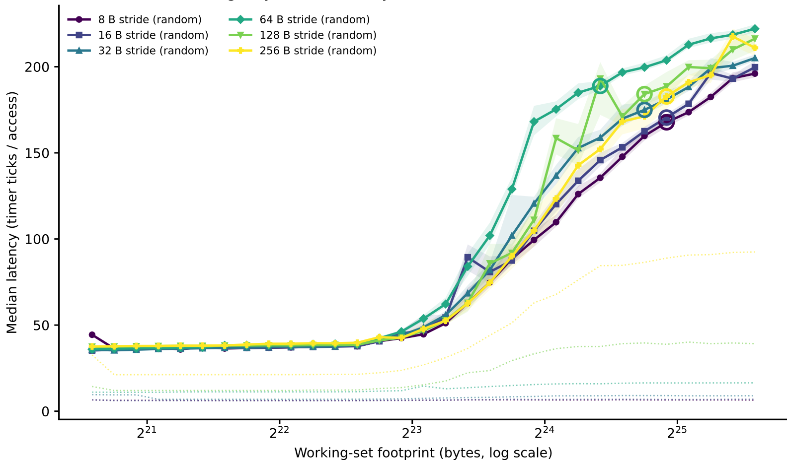
upgrade: line-size family of curves (dependent pointer chase) (Phase I timing-only, level boundary=12582912B window=[1572864,50331648])
