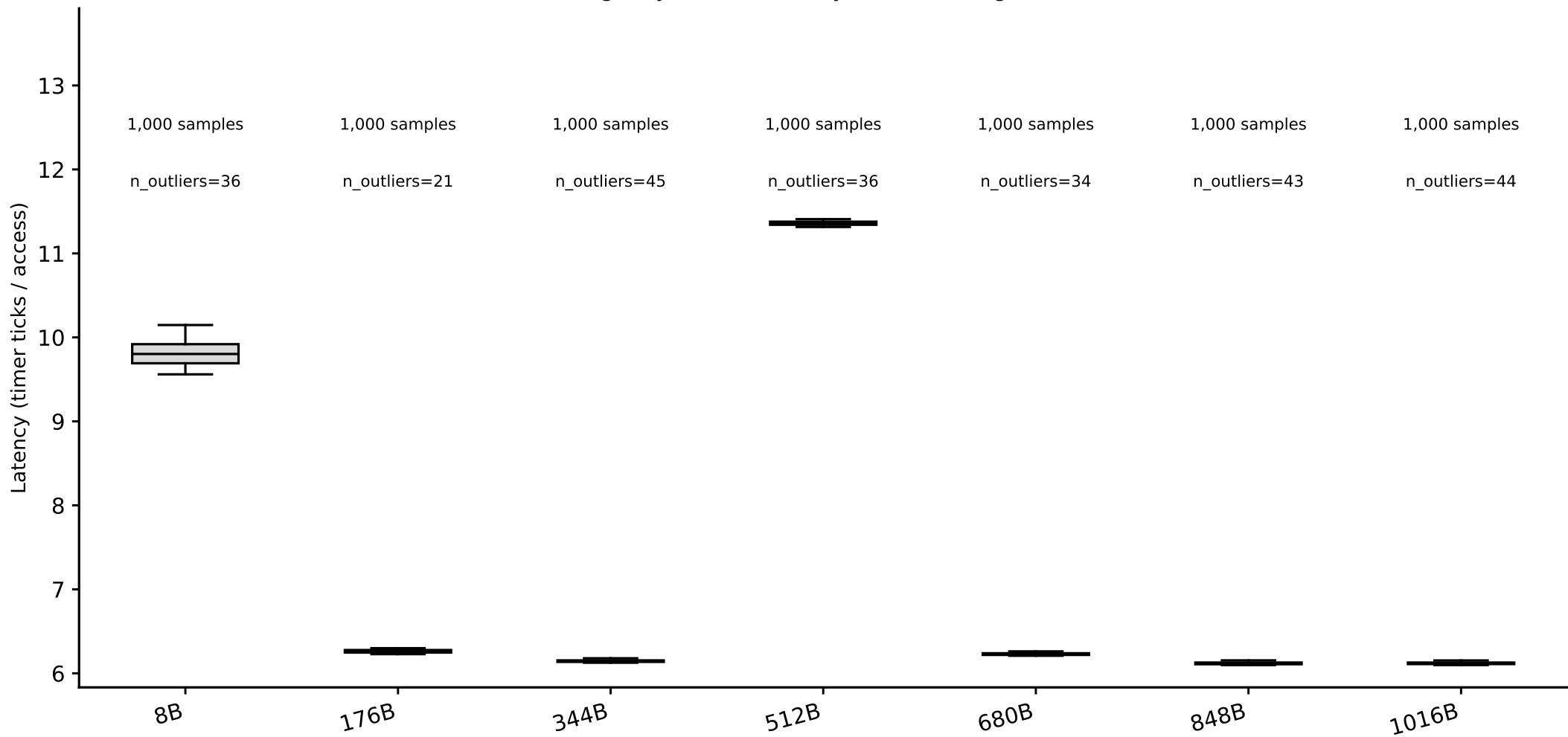
upgrade: line-size box plots, random pattern (whiskers = p5/p95) (Phase I timing-only, level boundary=32768B, single-curve method)
