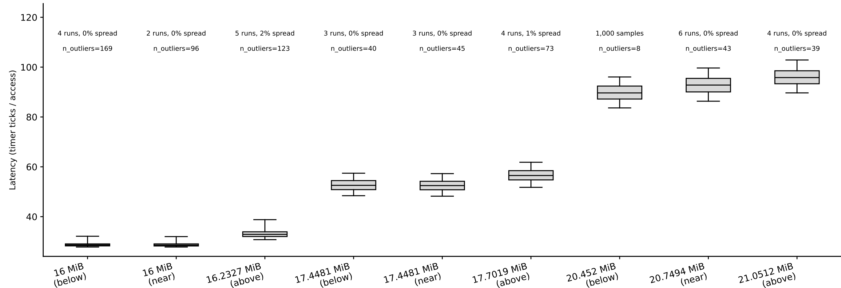
skylark: capacity box plots, random pattern (whiskers = p5/p95) (Phase I timing-only, extended to 2 GiB) tested boundaries: 16 MiB, 17.4481 MiB, 20.7494 MiB
