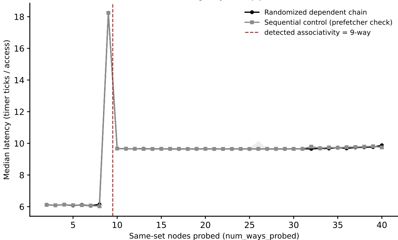
skylark: associativity sweep, L1 (stride=32 KiB) (Phase I timing-only, auto pipeline)
