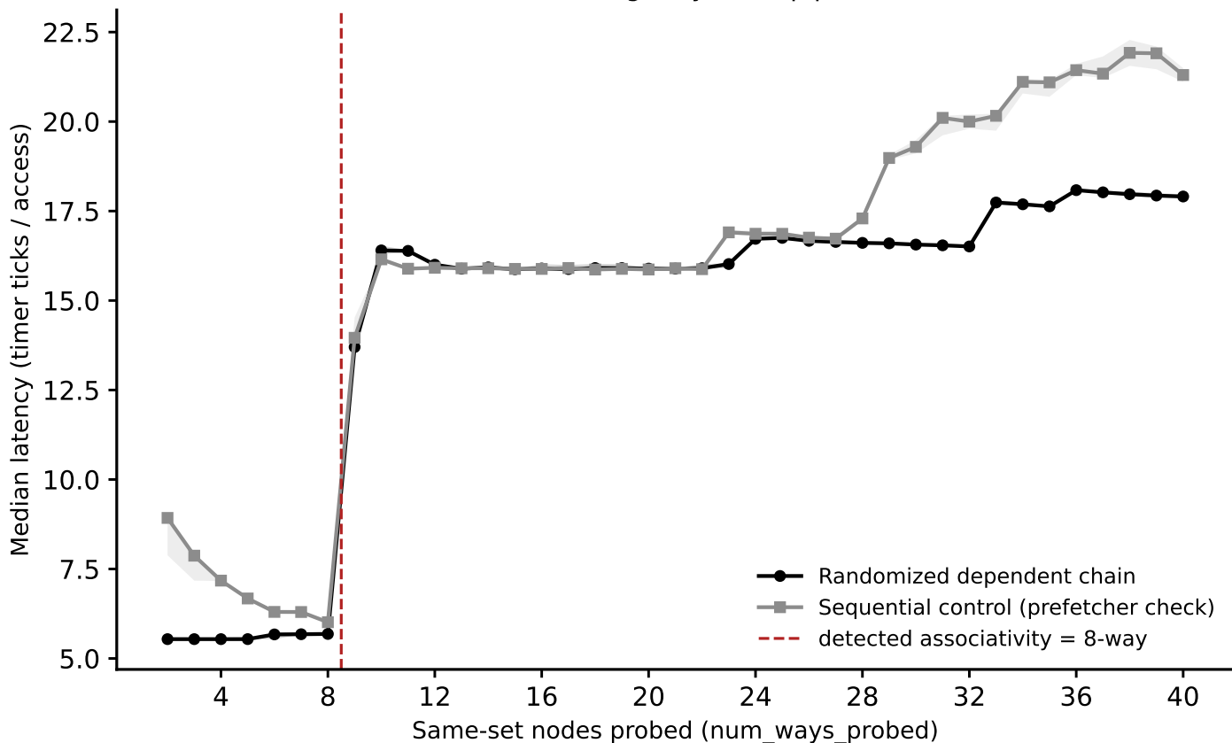
crux: associativity sweep, L1 (stride=32 KiB) (Phase I timing-only, auto pipeline)
