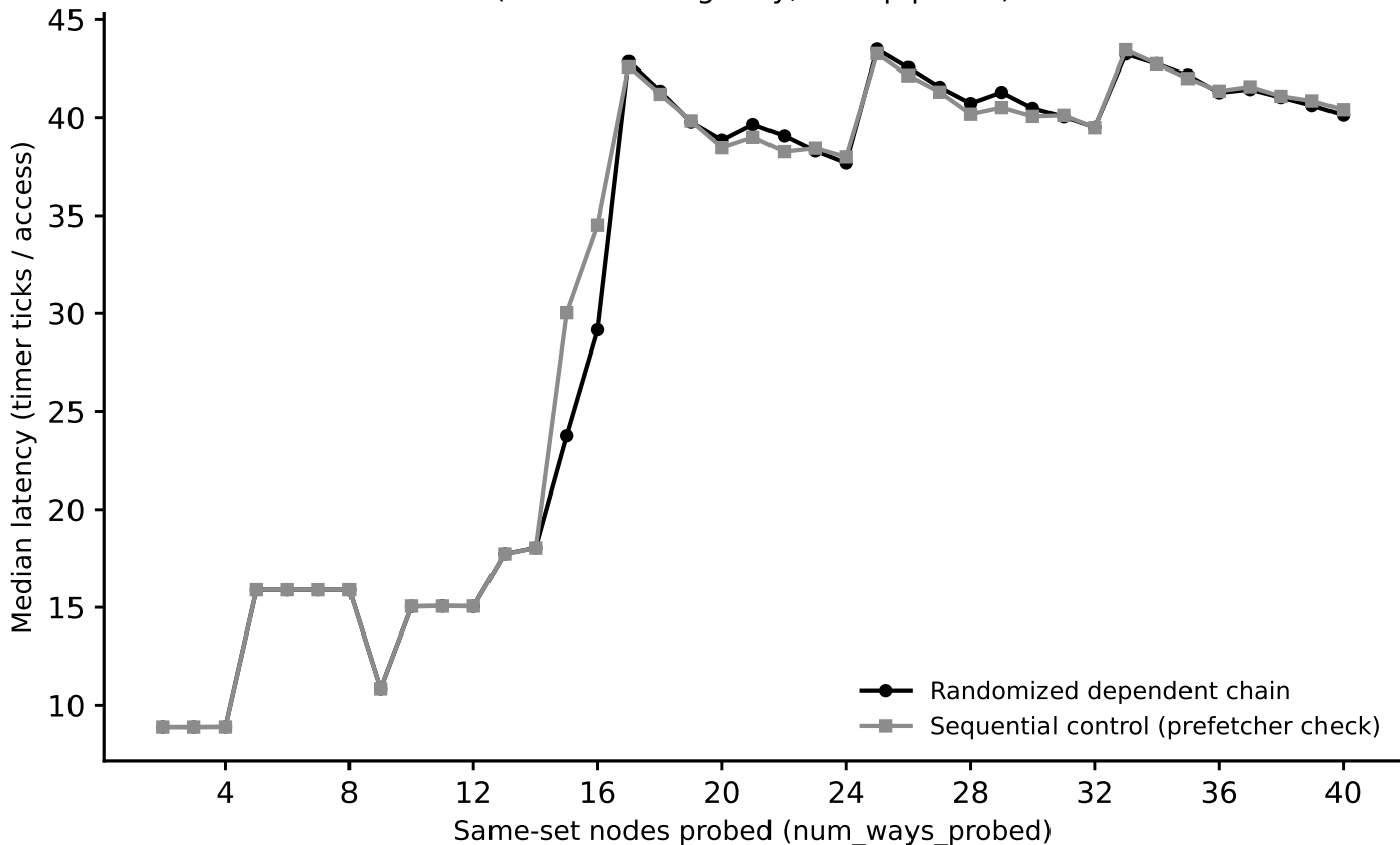
hazel_broadwell: associativity sweep, L2 (stride=256 KiB) (Phase I timing-only, auto pipeline)
