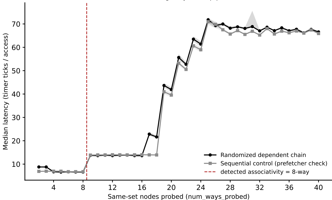
hazel_cascadelake/phase1_v2: associativity sweep, L2 (stride=1 MiB) (Phase I timing-only, auto pipeline)
