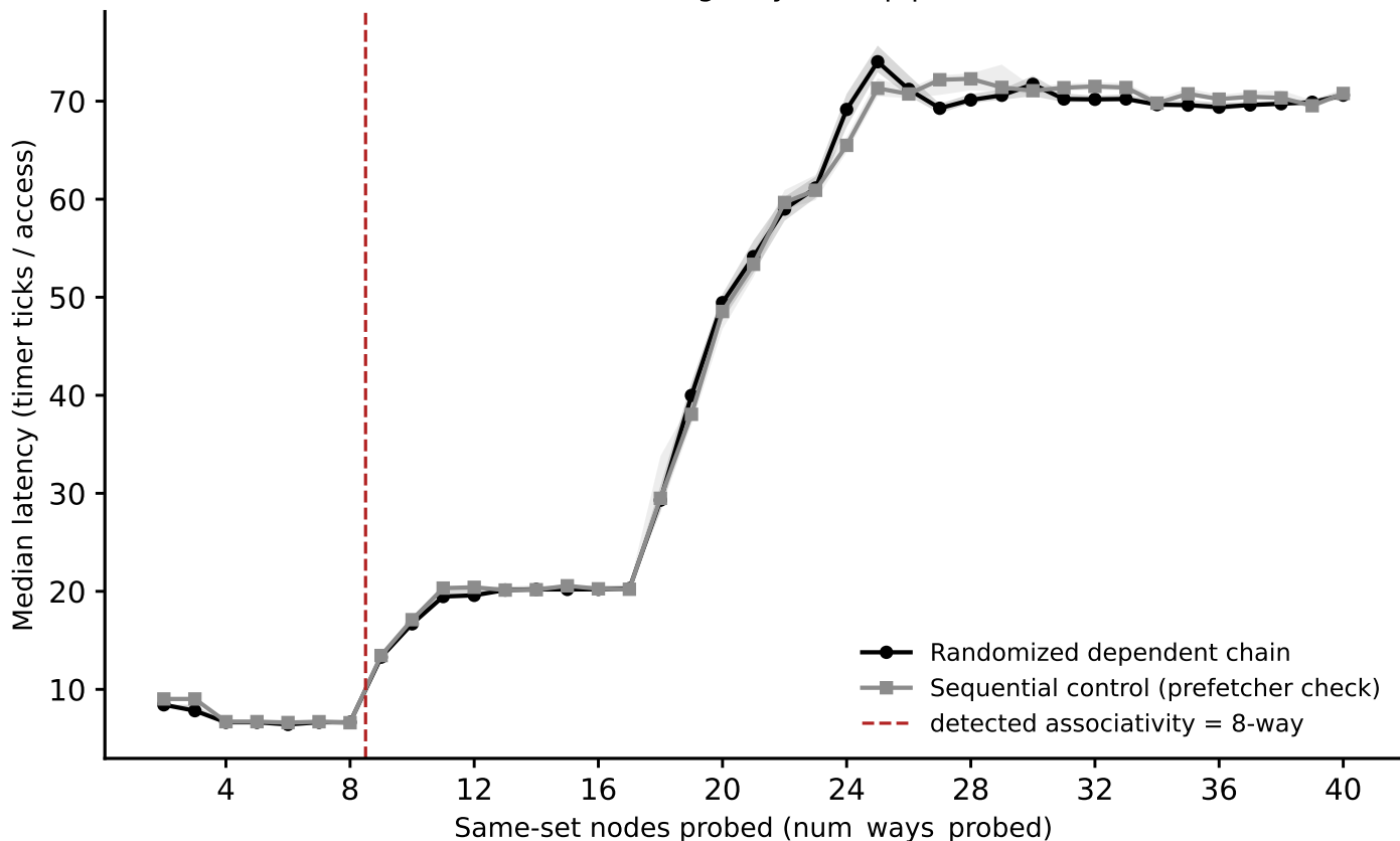
hazel_cascadelake/phase1_v2: associativity sweep, L3_LLC (stride=16 MiB) (Phase I timing-only, auto pipeline)
