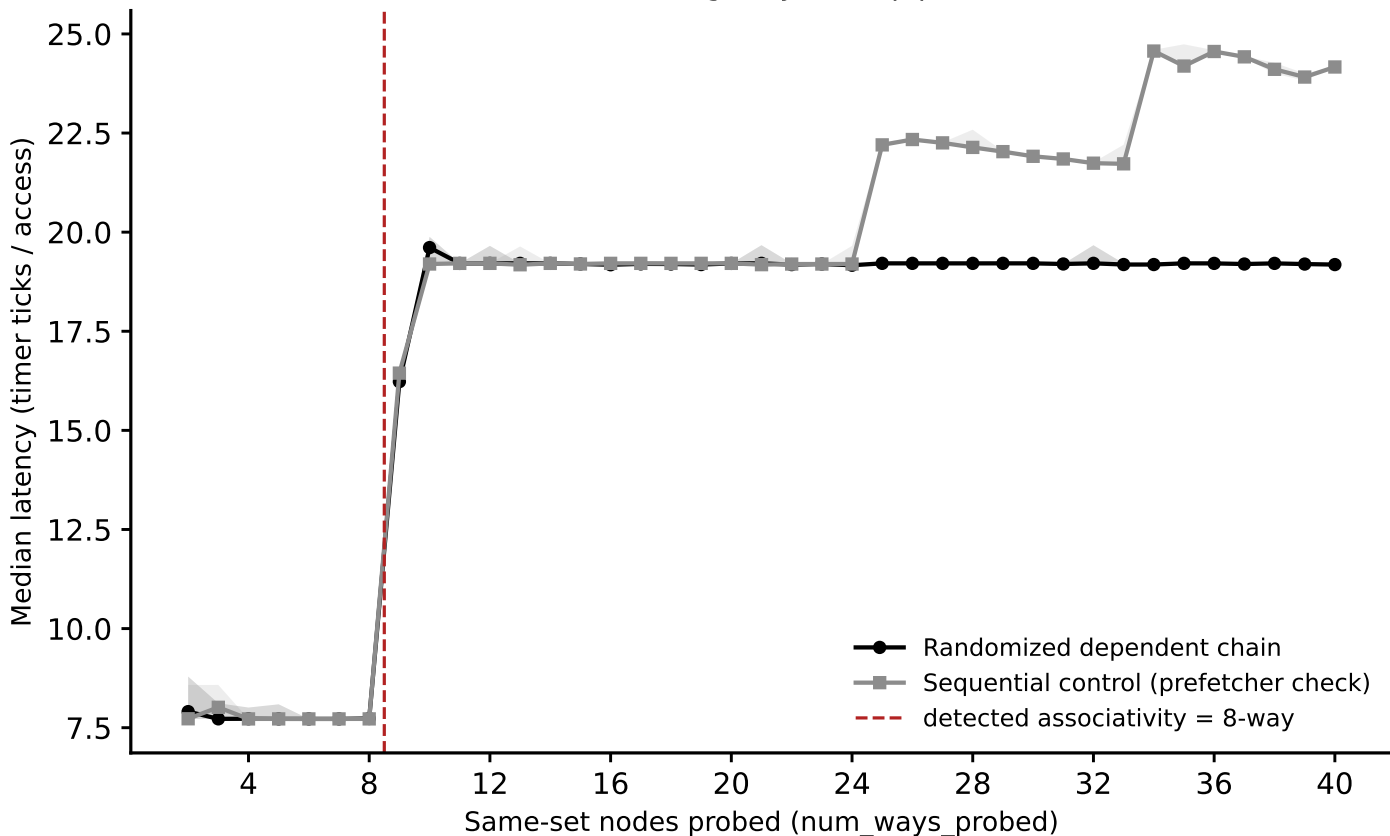
hazel_haswell: associativity sweep, L1 (stride=32 KiB) (Phase I timing-only, auto pipeline)
