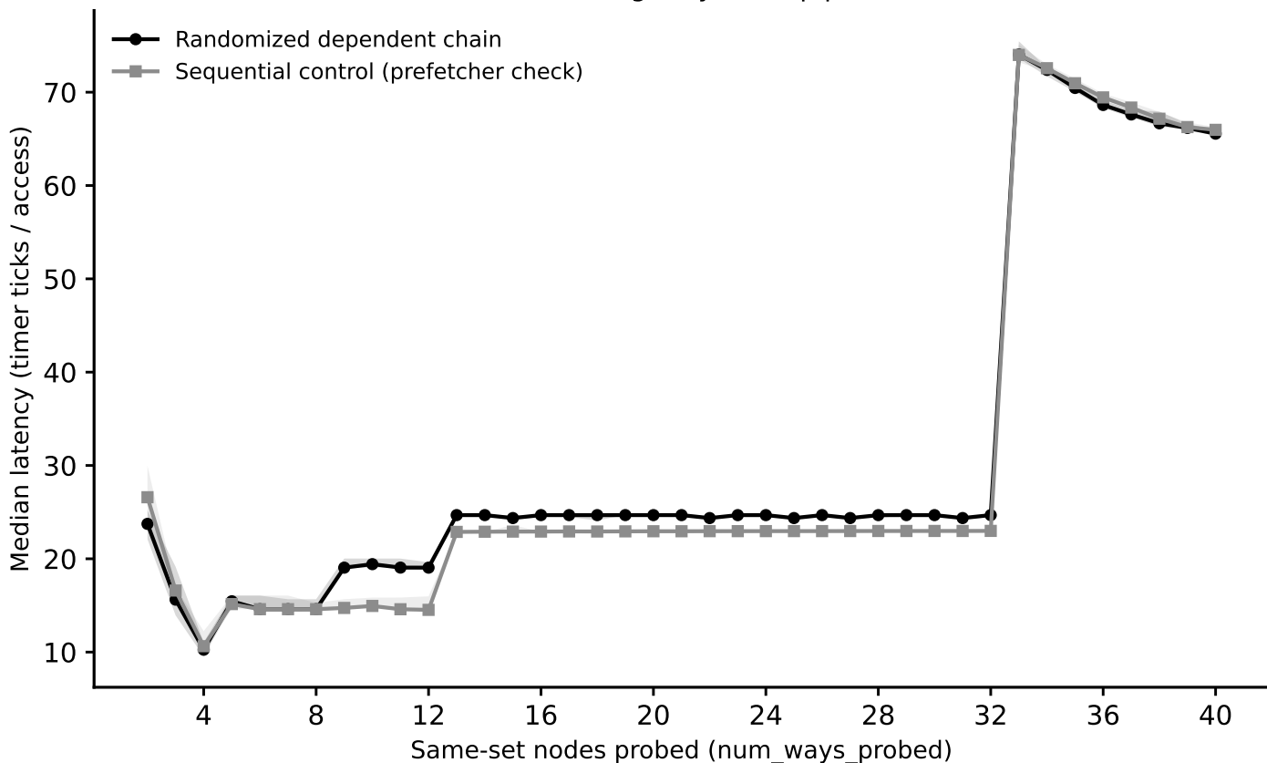
hazel_icelake_6326/phase1_v2: associativity sweep, L1 (stride=64 KiB) (Phase I timing-only, auto pipeline)
