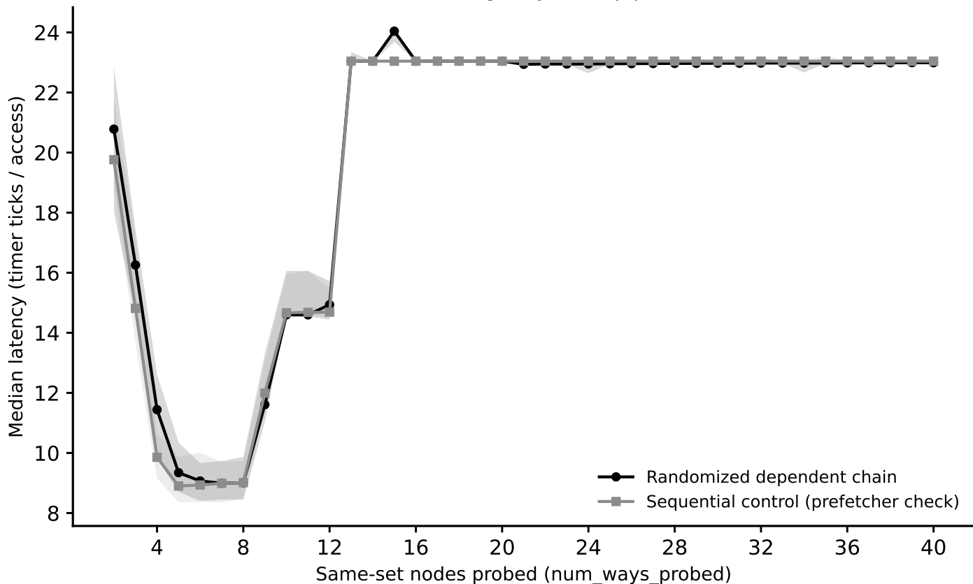
hazel_icelake_8358: associativity sweep, L1 (stride=32 KiB) (Phase I timing-only, auto pipeline)
