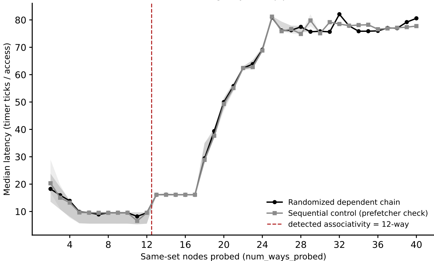
hazel_sapphirerapids/phase1_v2: associativity sweep, L2 (stride=2 MiB) (Phase I timing-only, auto pipeline)
