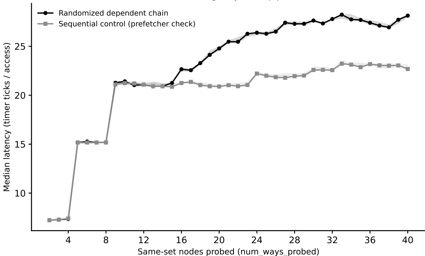
ookay: associativity sweep, L2 (stride=256 KiB) (Phase I timing-only, auto pipeline)
