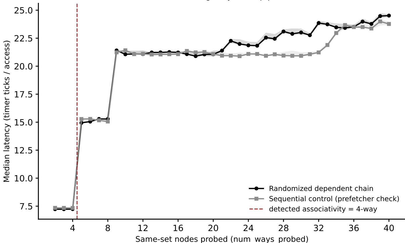
ookay: associativity sweep, L3_LLC (stride=8 MiB) (Phase I timing-only, auto pipeline)
