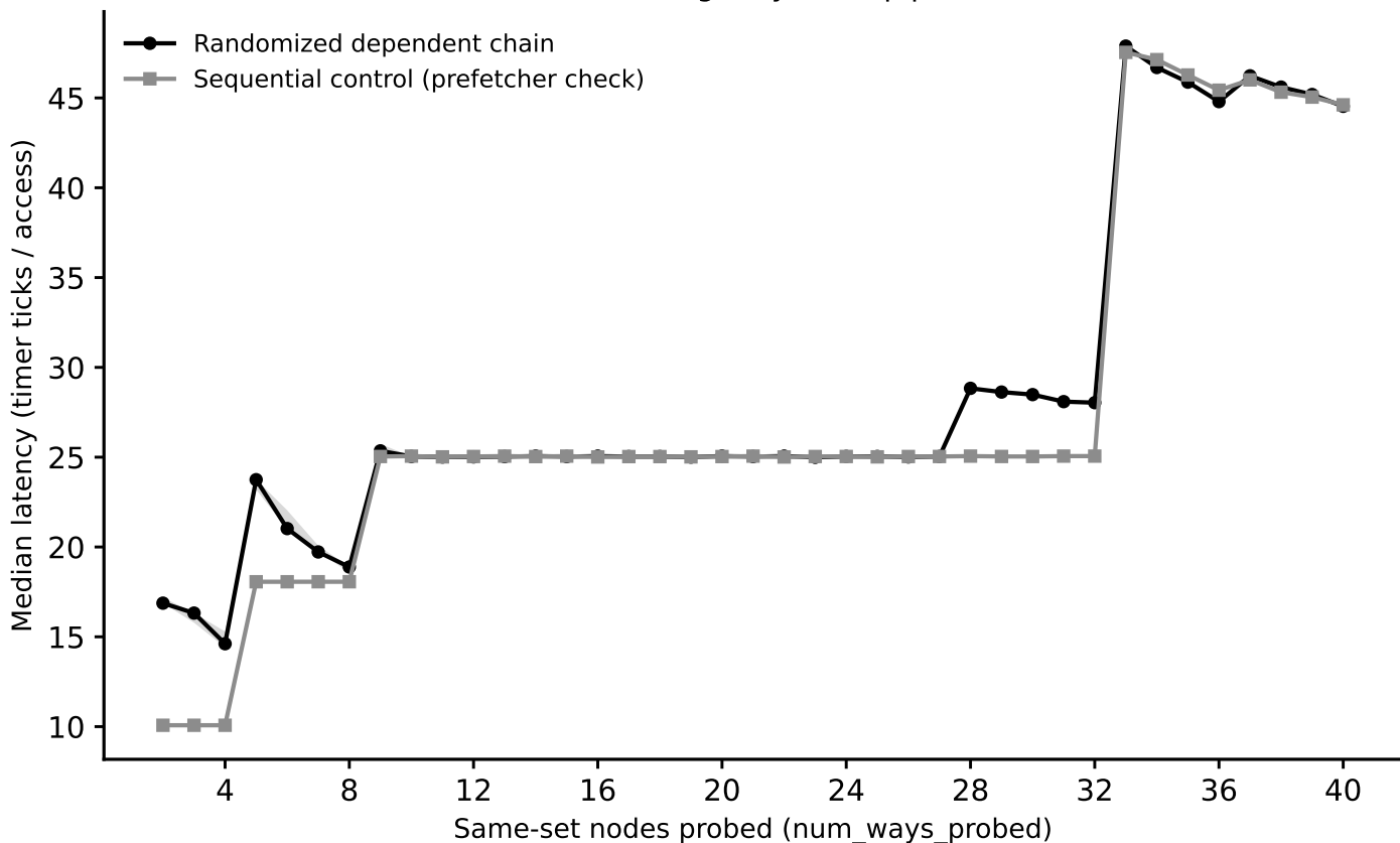
sunbird: associativity sweep, L2_2MiB_candidate (stride=64 KiB) (Phase I timing-only, auto pipeline)
