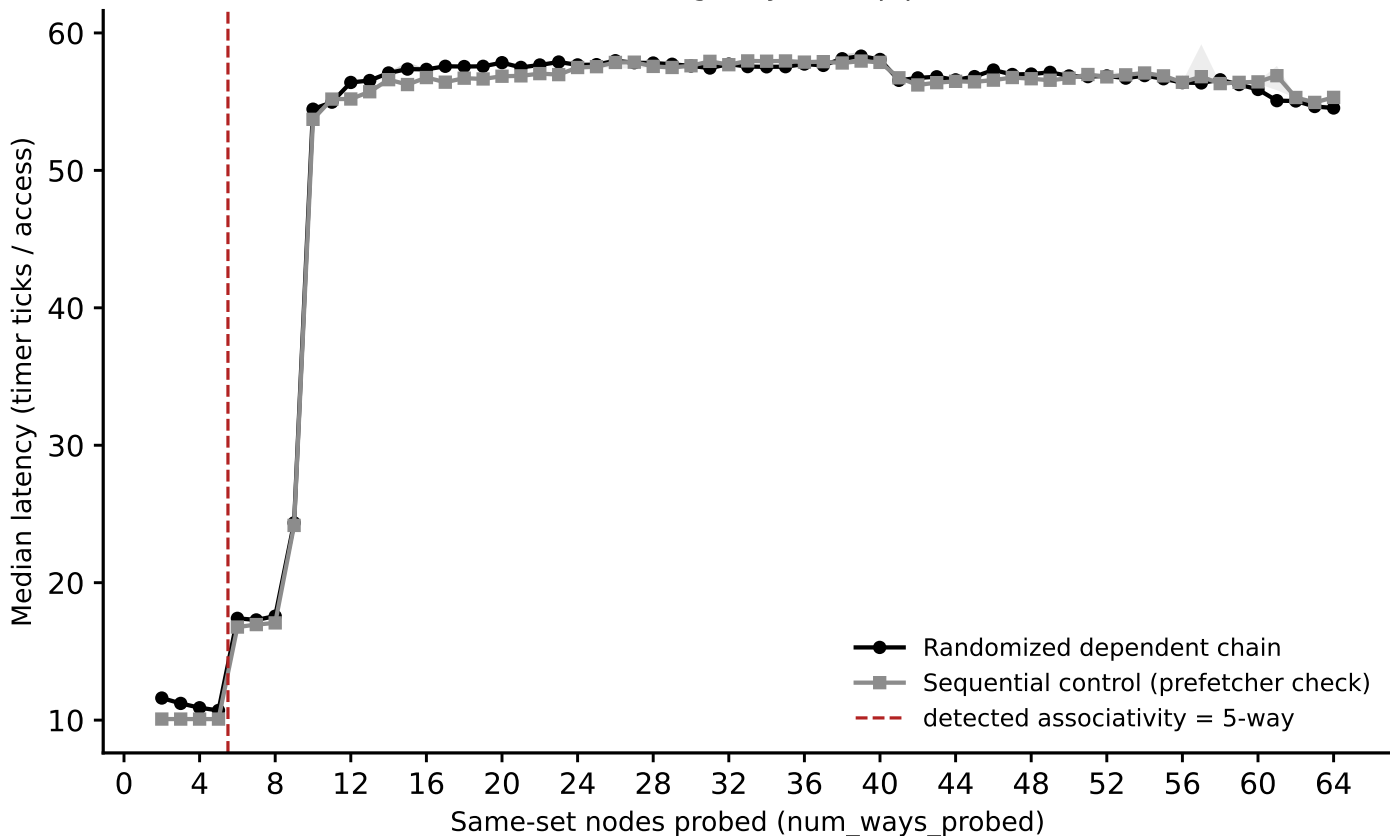
sunbird: associativity sweep, LLC_32MiB (stride=32 MiB) (Phase I timing-only, auto pipeline)
