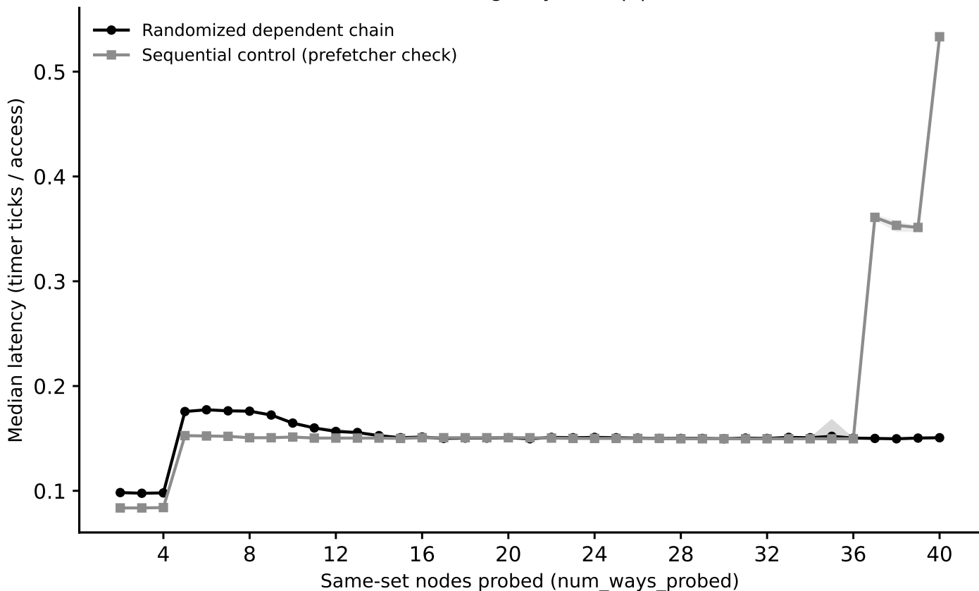
thunderbird: associativity sweep, L1 (stride=64 KiB) (Phase I timing-only, auto pipeline)
