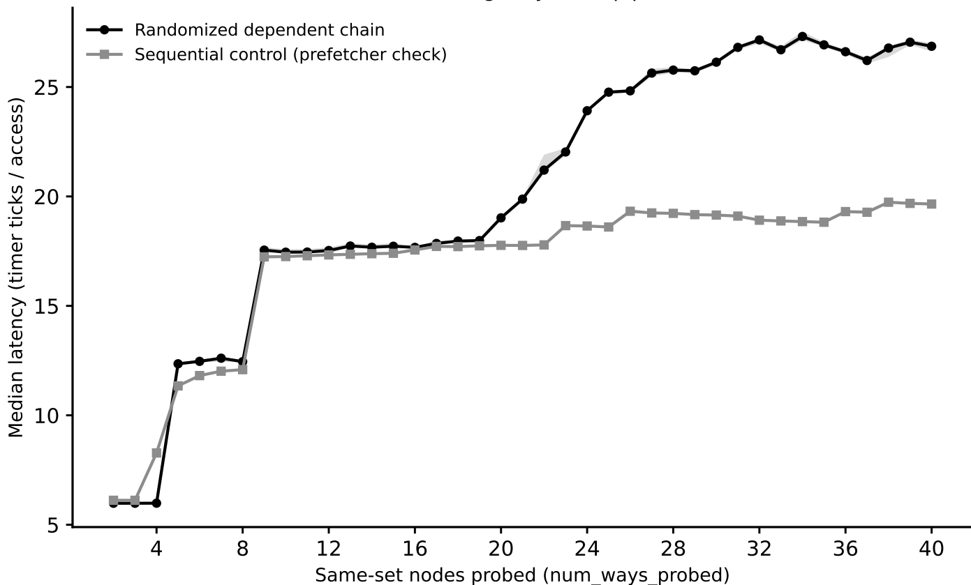
upgrade: associativity sweep, L2 (stride=256 KiB) (Phase I timing-only, auto pipeline)
