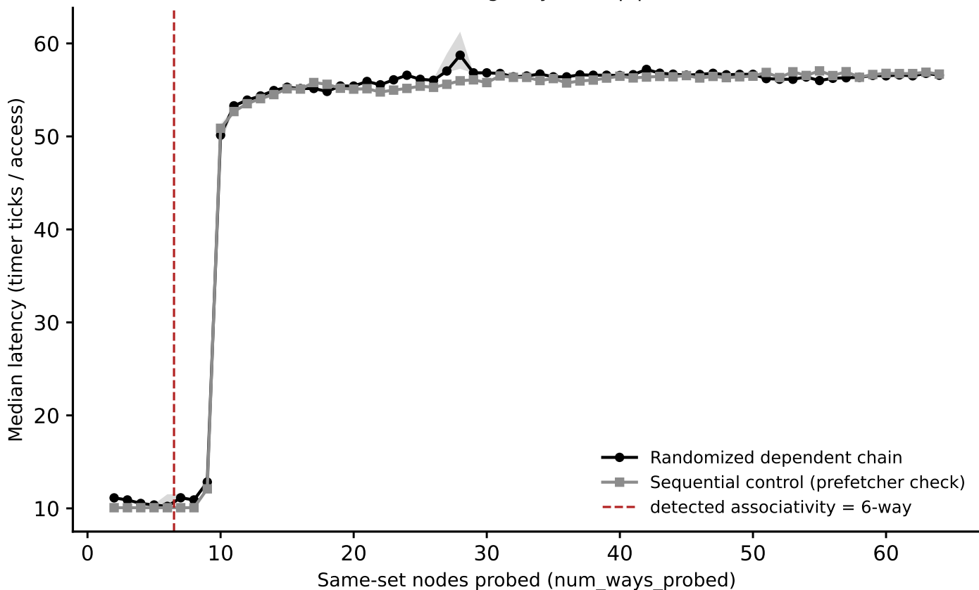
sunbird: associativity sweep, L1 (stride=16 MiB) (Phase I timing-only, auto pipeline)
