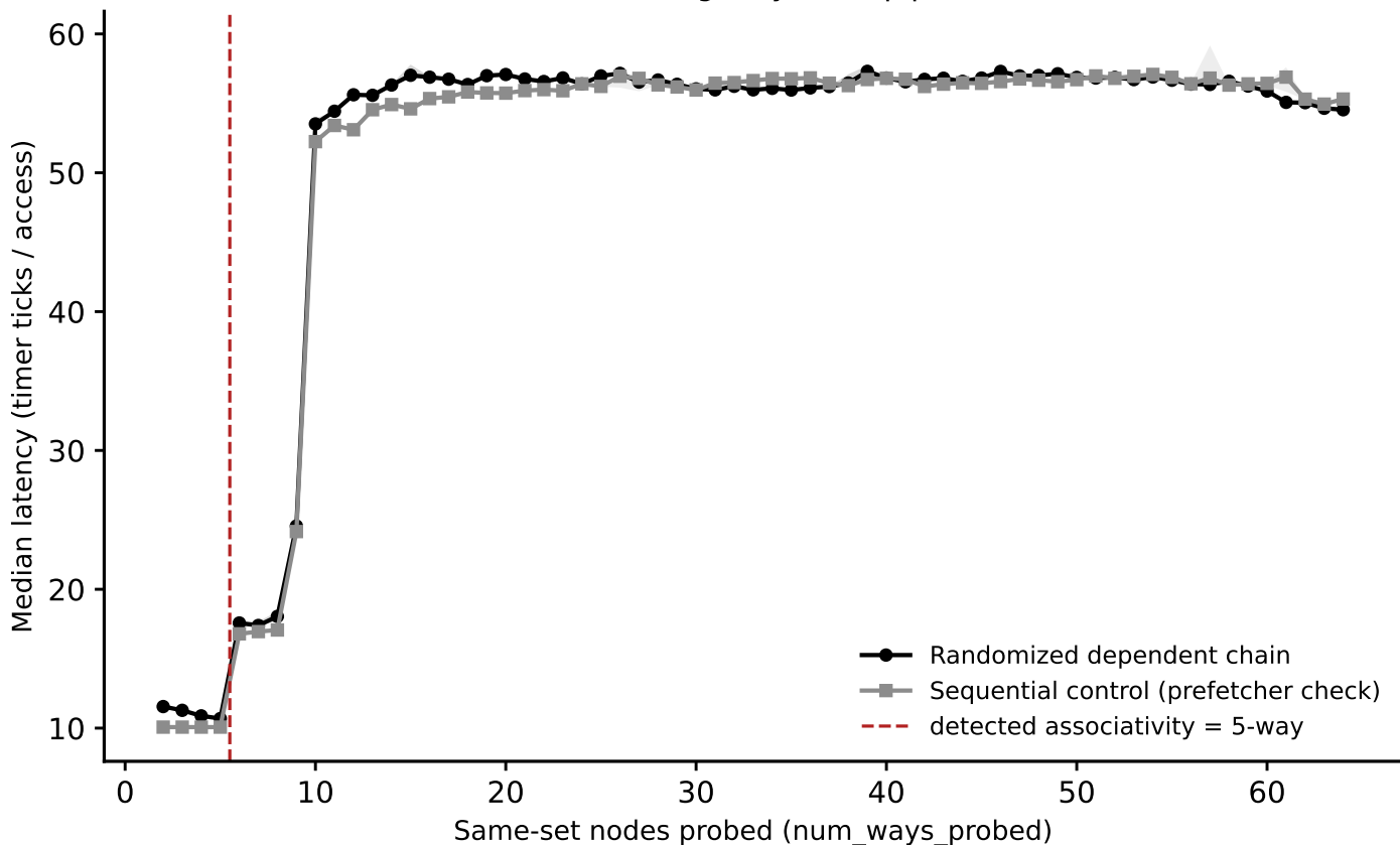
sunbird: associativity sweep, L1 (stride=32 MiB) (Phase I timing-only, auto pipeline)
