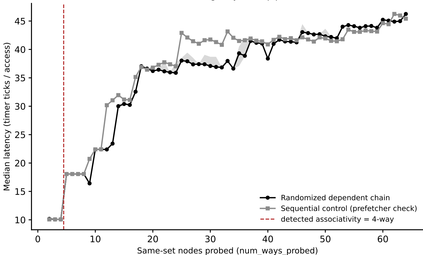
sunbird: associativity sweep, L1 (stride=256 KiB) (Phase I timing-only, auto pipeline)
