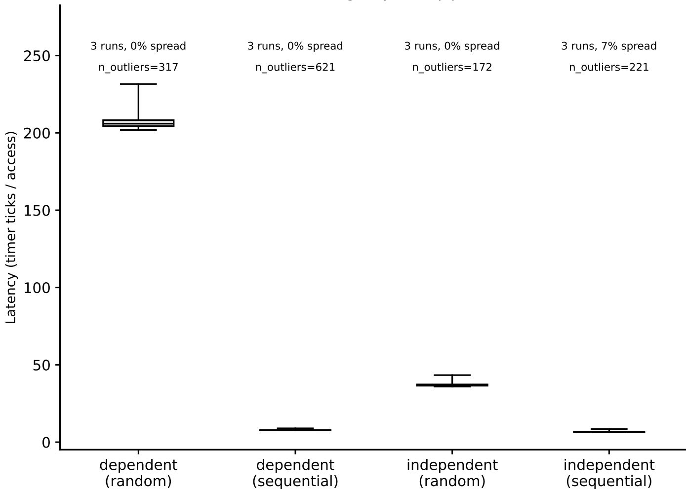
hazel_haswell: hit-latency box plots, DRAM (footprint=512 MiB) (Phase I timing-only, auto pipeline)
