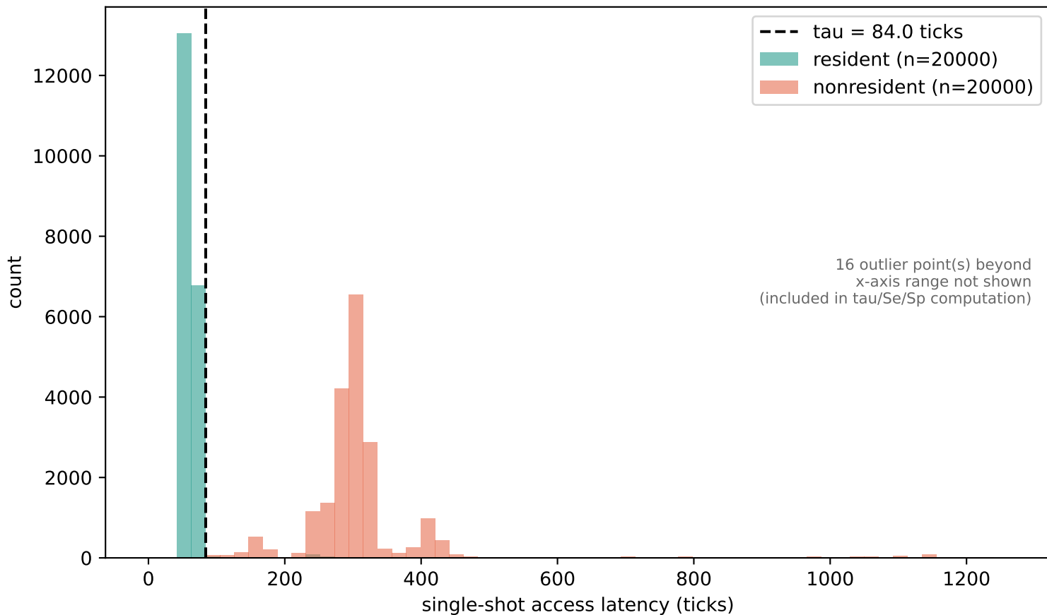
Calibration distributions: resident vs. nonresident (sunbird)
