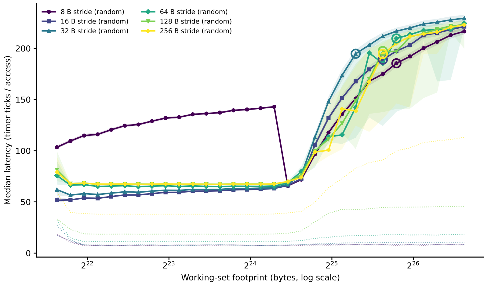
hazel_icelake_6326/line_size_rerun: line-size family of curves (dependent pointer chase) (Phase I timing-only, level boundary=25874000B window=[3234250,103496000])
