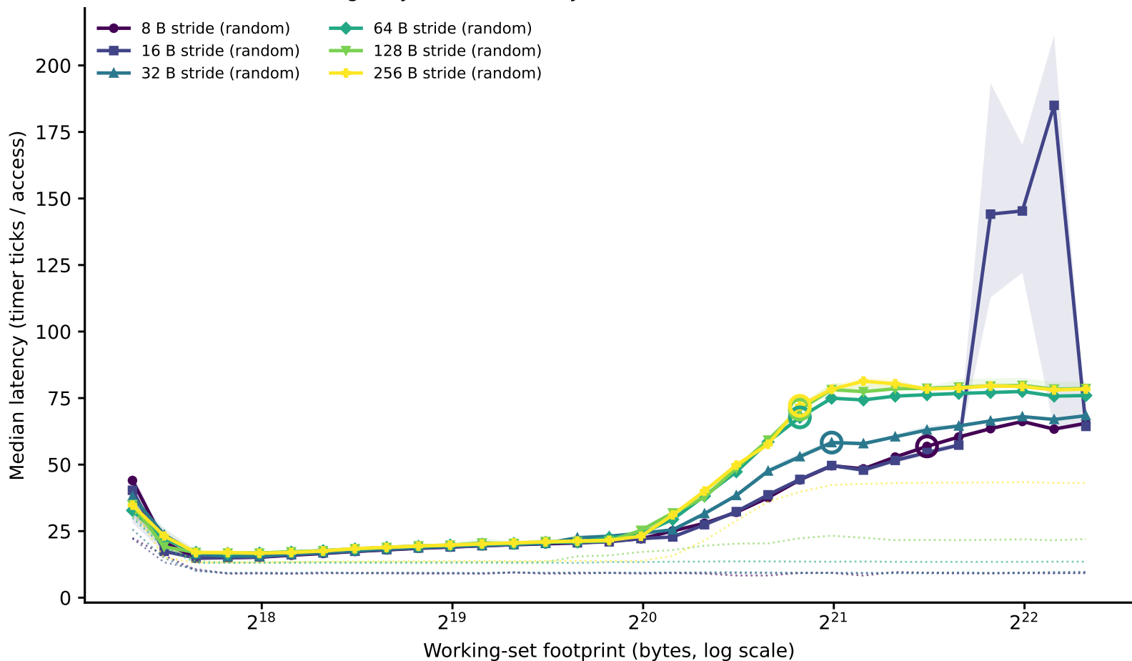
hazel_icelake_8358/line_size_rerun: line-size family of curves (dependent pointer chase) (Phase I timing-only, level boundary=1310720B window=[163840,524288])
