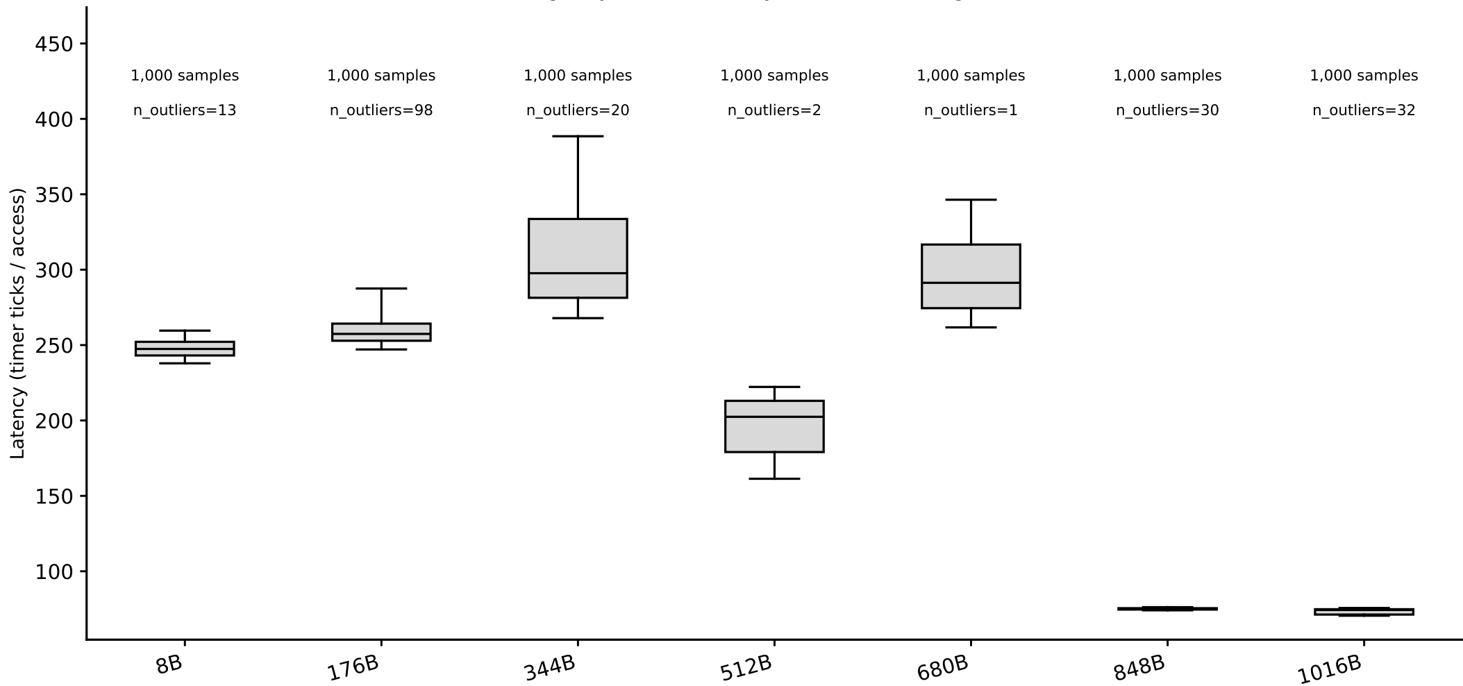
hazel_icelake_8358/line_size_rerun: line-size box plots, random pattern (whiskers = p5/p95) (Phase I timing-only, level boundary=50331648B, single-curve method)
