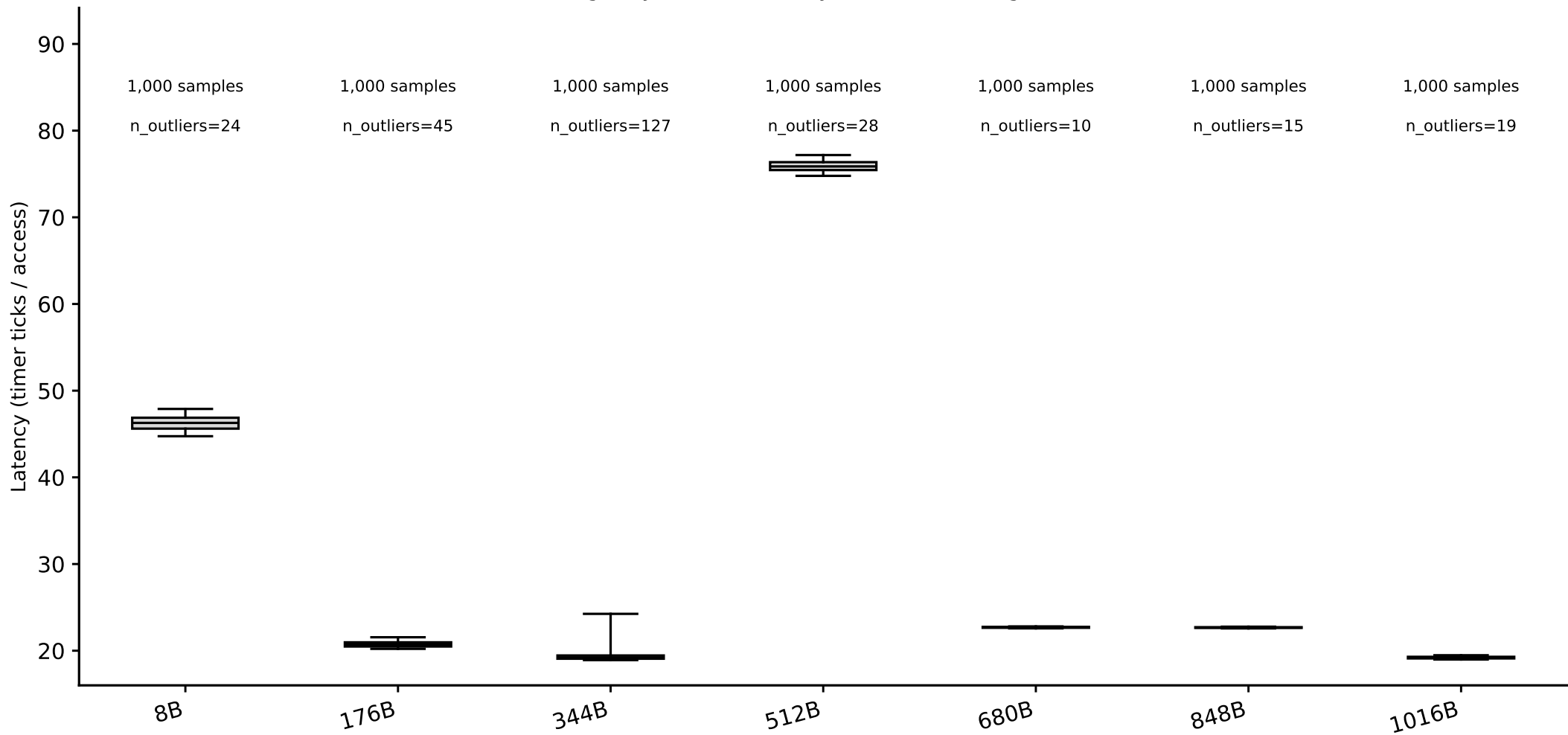
hazel_sapphirerapids/line_size_rerun: line-size box plots, random pattern (whiskers = p5/p95) (Phase I timing-only, level boundary=2097152B, single-curve method)
