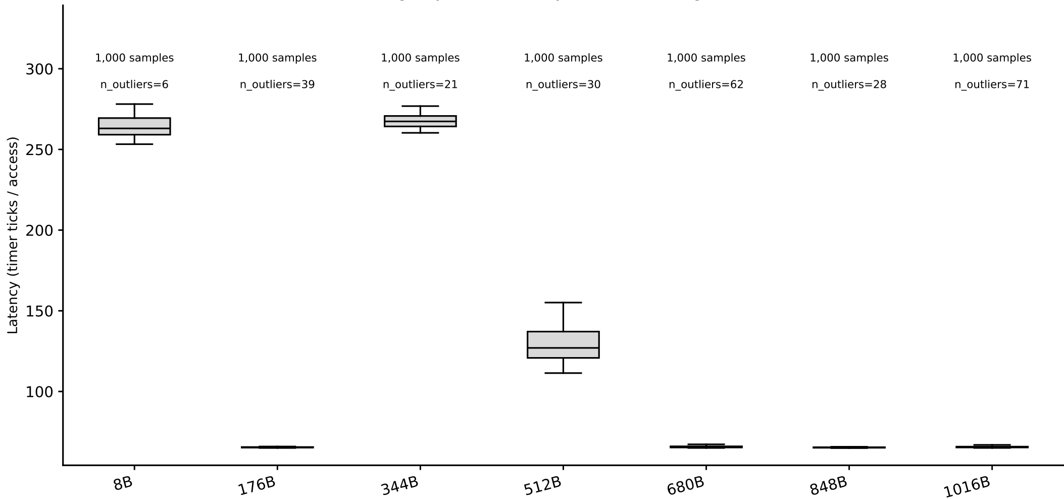
hazel_sapphirerapids/line_size_rerun: line-size box plots, random pattern (whiskers = p5/p95) (Phase I timing-only, level boundary=39903168B, single-curve method)
