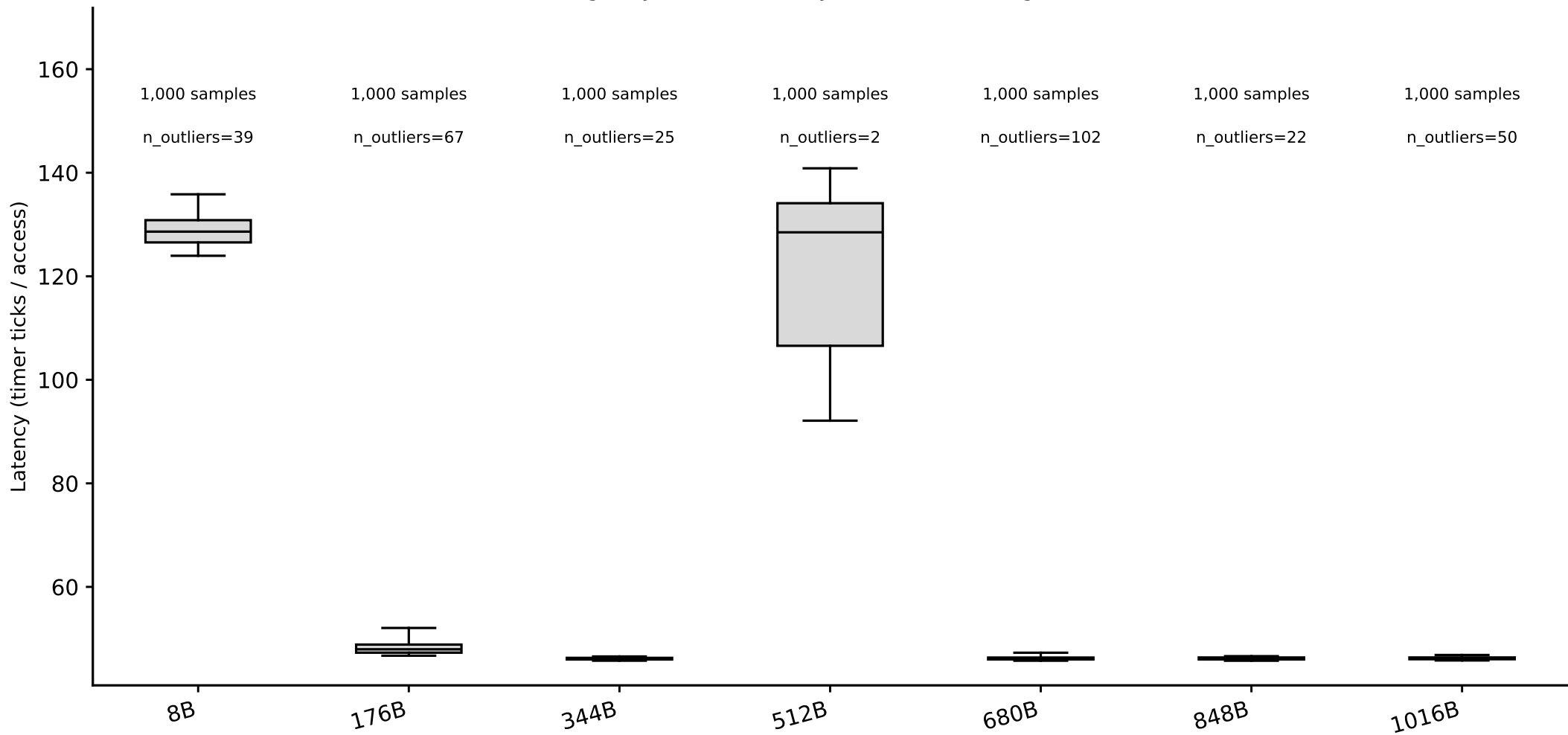
hazel_skylake/line_size_rerun: line-size box plots, random pattern (whiskers = p5/p95) (Phase I timing-only, level boundary=23726560B, single-curve method)
