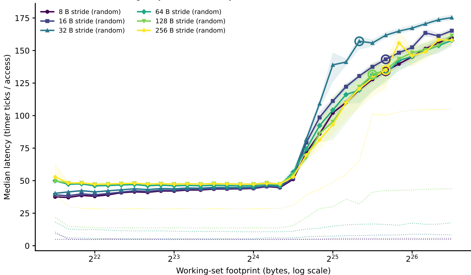
hazel_skylake/line_size_rerun: line-size family of curves (dependent pointer chase) (Phase I timing-only, level boundary=23726560B window=[2965820,94906240])
