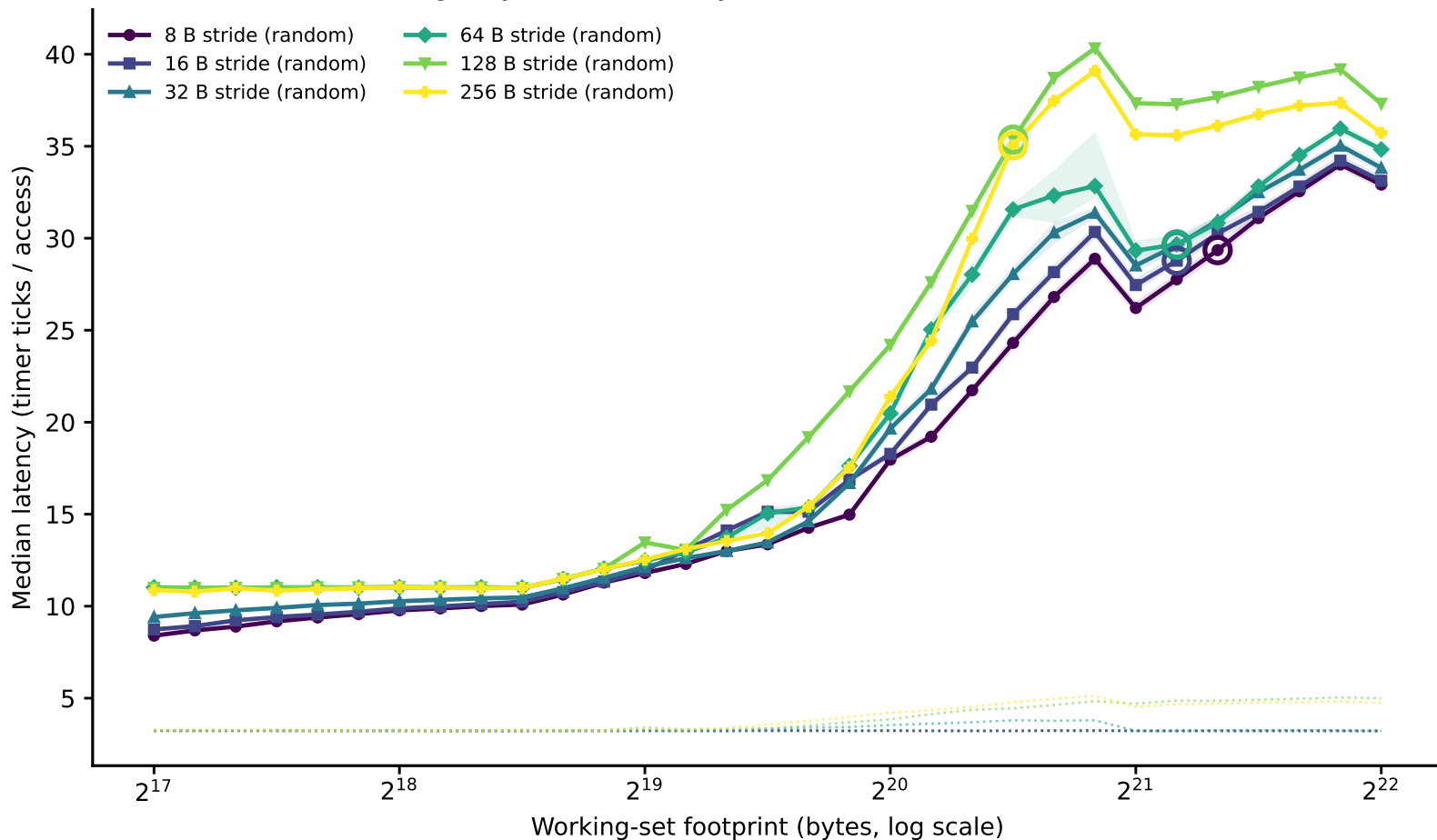
hazel_turin/line_size_rerun: line-size family of curves (dependent pointer chase) (Phase I timing-only, level boundary=1048576B window=[131072,4194304])
