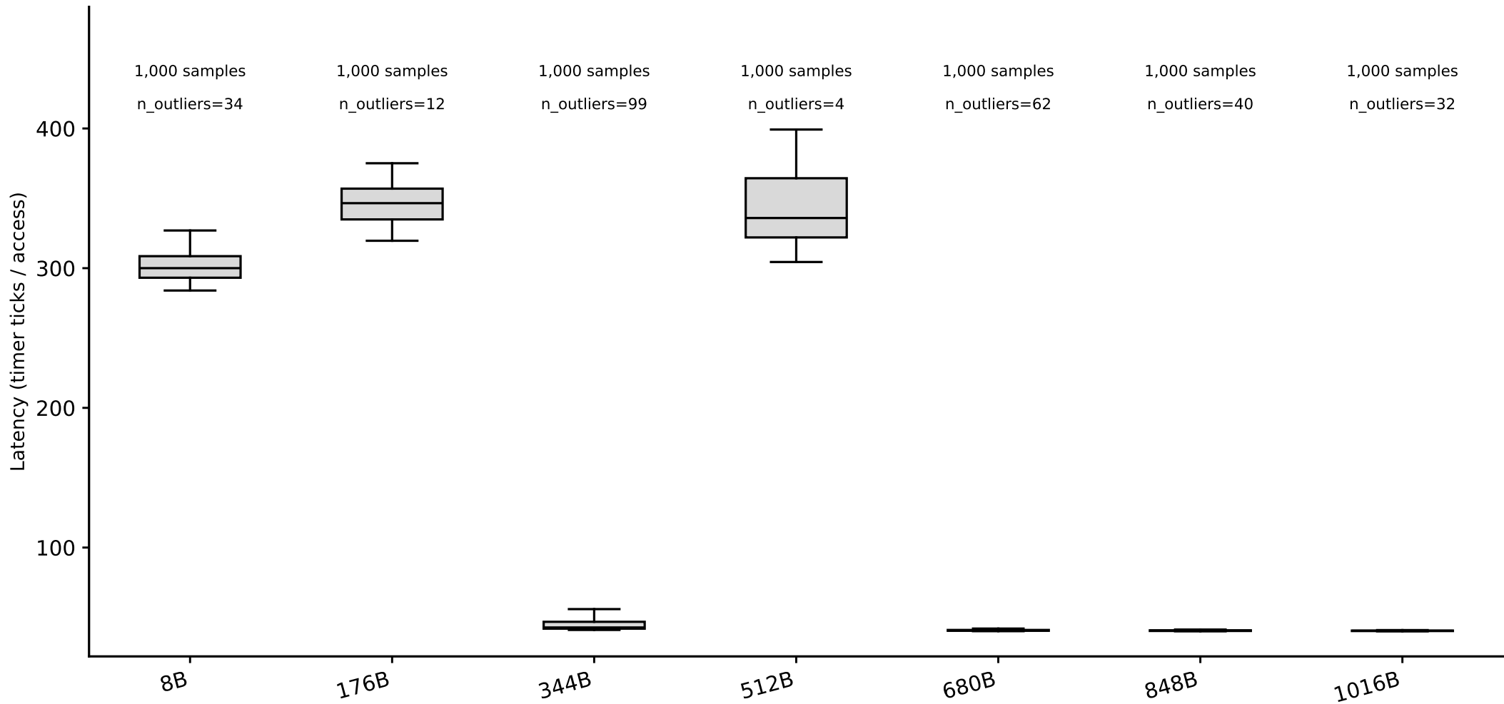
hazel_turin/line_size_rerun: line-size box plots, random pattern (whiskers = p5/p95) (Phase I timing-only, level boundary=33554432B, single-curve method)
