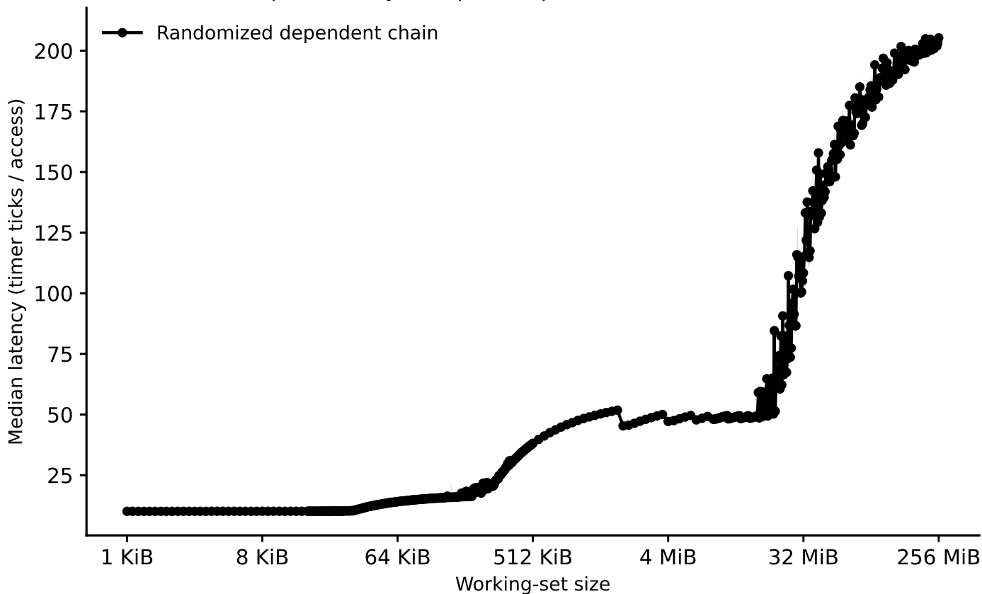
sunbird: capacity sweep (dependent pointer chase) (random pattern only -- sequential prefetcher-check control omitted)
