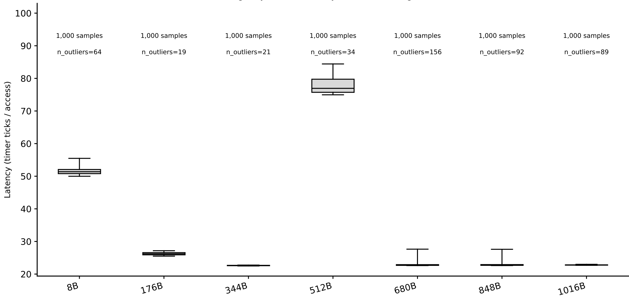
artemis: line-size box plots, random pattern (whiskers = p5/p95) (Phase I timing-only, level boundary=2097152B, single-curve method)
