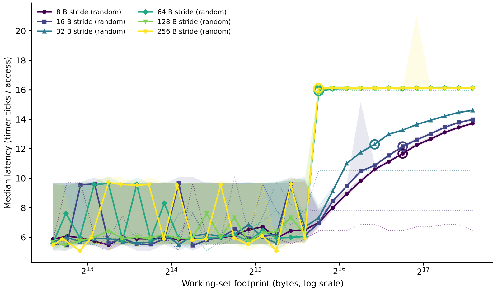
artemisia: line-size family of curves (dependent pointer chase) (Phase I timing-only, level boundary=49152B window=[6144,196608])
