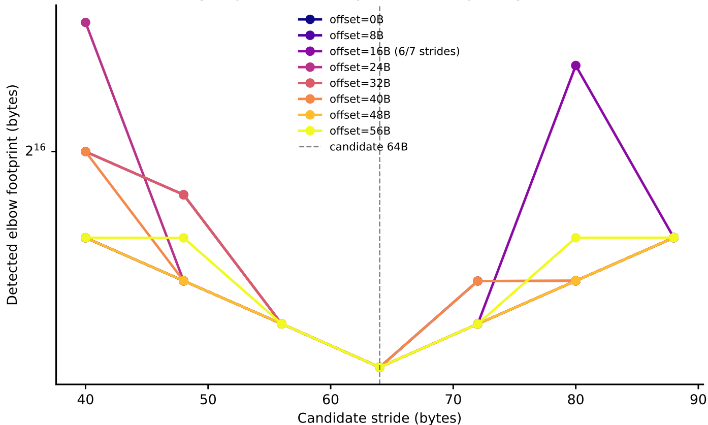
charnwood: line-size elbow vs. stride, by node-0 offset (Phase I timing-only, level boundary=32768B, step-4 alignment refinement)
