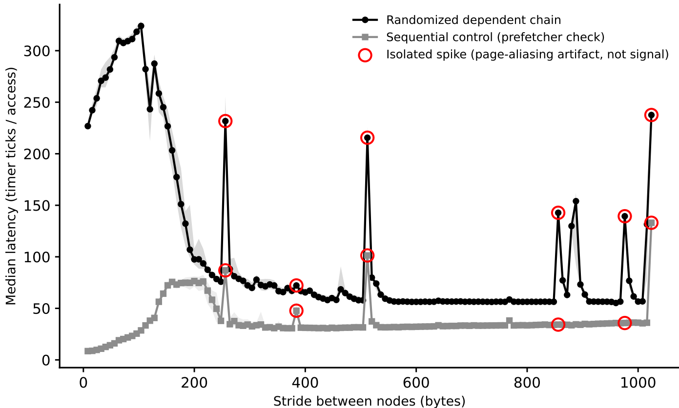
charnwood: line-size sweep (dependent pointer chase), footprint=16 MiB (Phase I timing-only, level boundary=8388608B, single-curve method)
